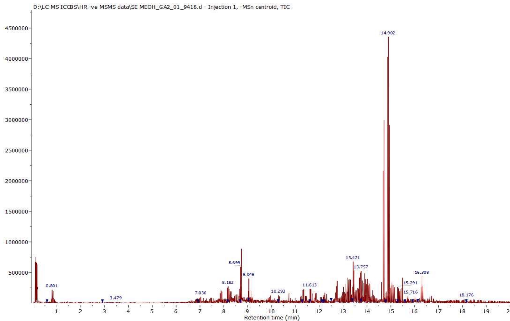
Figure . Total ion chromatogram of the methanolic extract. SAE.
