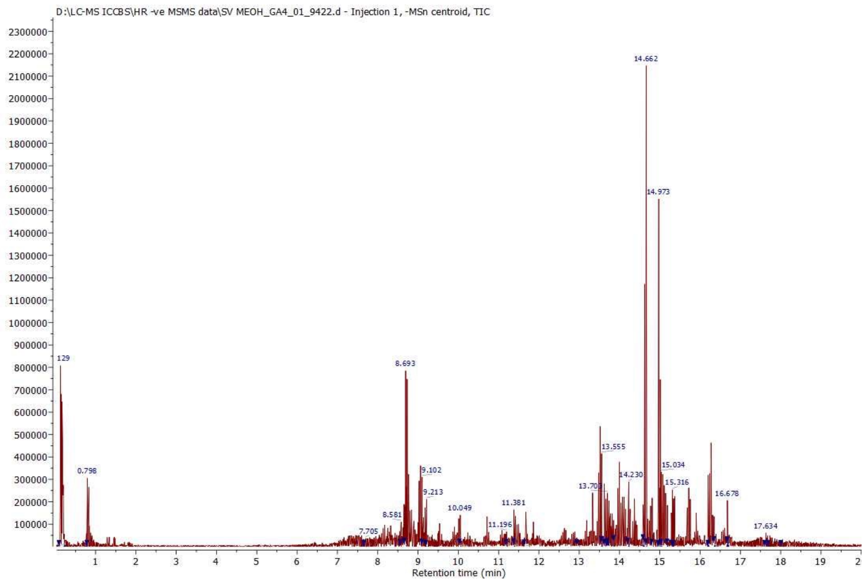
Figure Total ion chromatogram of the methanolic extract. SVR.
