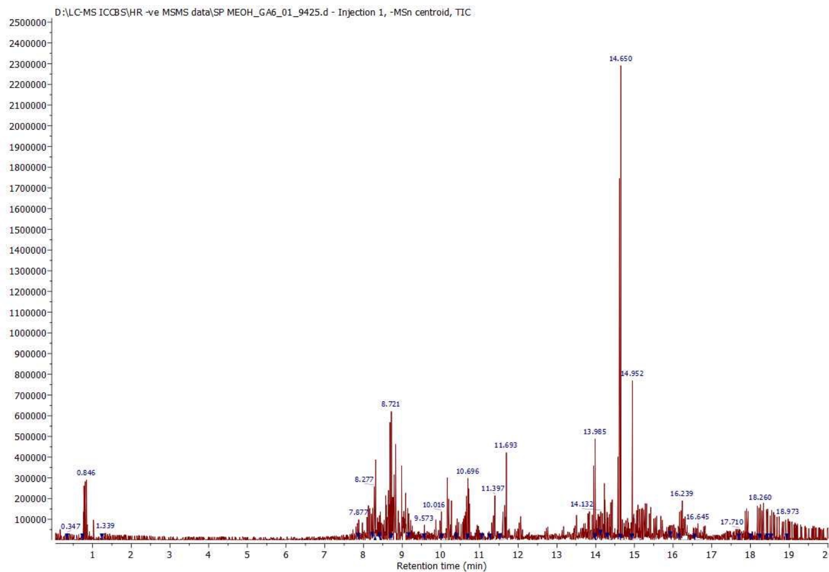
Figure Total ion chromatogram of SBA methanolic extract
