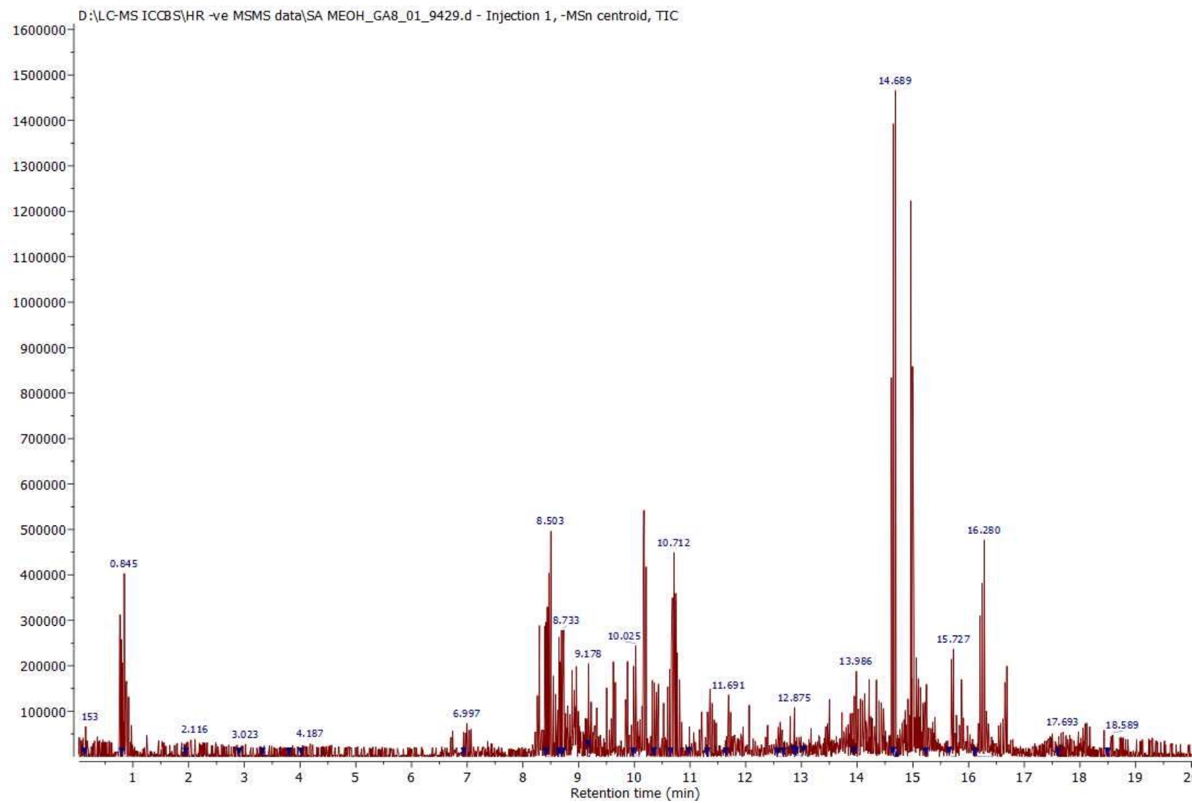
Figure Total ion chromatogram of the methanolic extract. SAR
